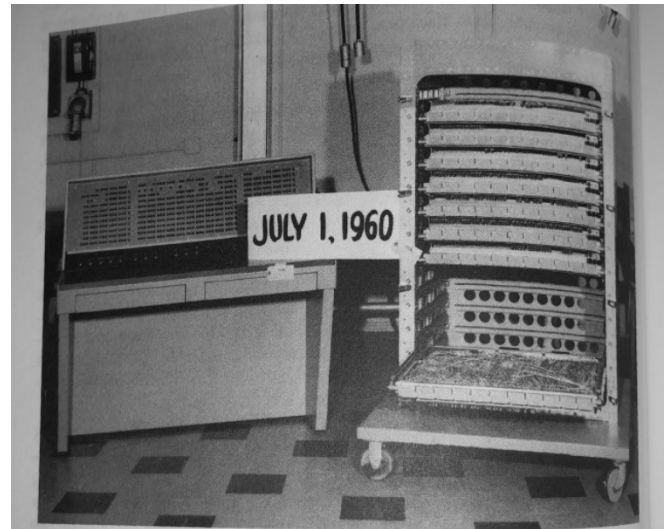
Figure 6.2: CP-642 NTDS unit computer serial number XN-1 in assembly at the Univac plant. Circuit cards can be seen inserted in the top seven drawers. The bottom drawer has been pulled out and inverted to reveal the dense point-to-point wiring among the circuit card connectors. Photo from Donald L. Ream, courtesy of Unisys.
