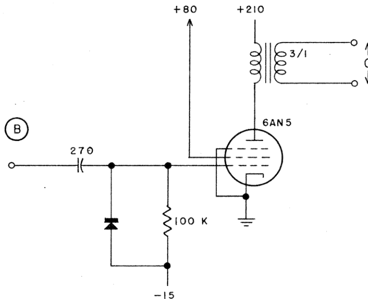
Figure 3 - Pulse Amplifier
