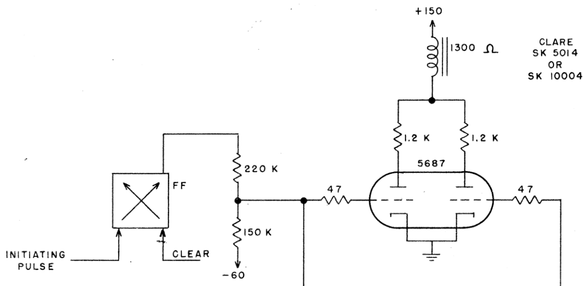
Figure 8 - Flip-flop and Relay Puller
