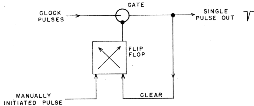
Figure 5 - Elementary Synchronizing Circuit
