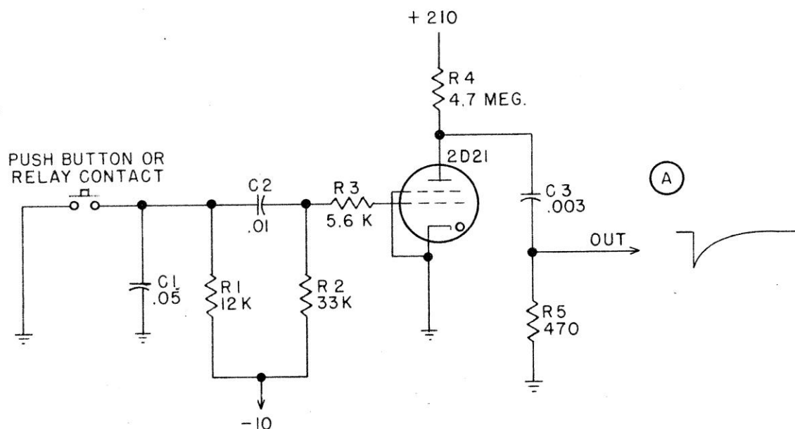
Figure 1 - Pulse-former
