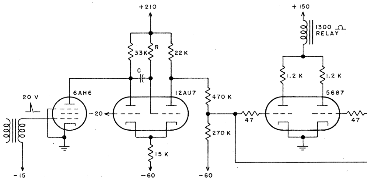
Figure 9 - One-Shot Multivibrator and Relay Puller
