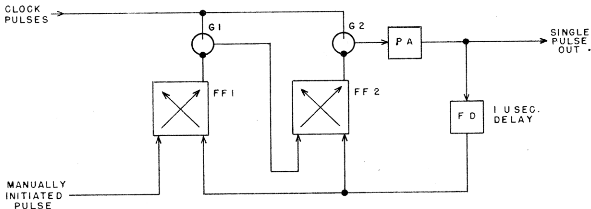
Figure 6 - Synchronizing Circuit
