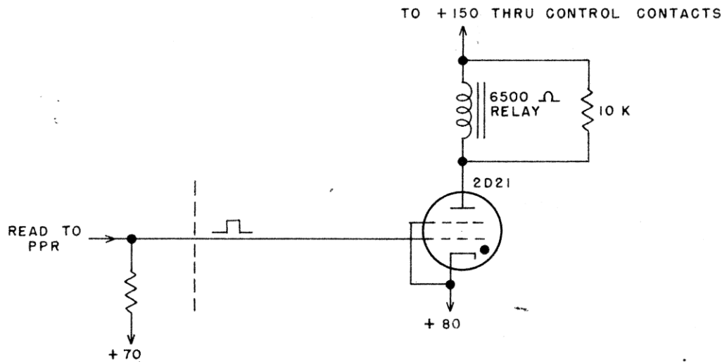
Figure 11 - Print Initiate Circuit
